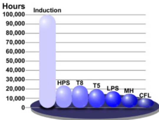
Lamp Life Comparison
