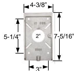
Mounting Plate Detail
