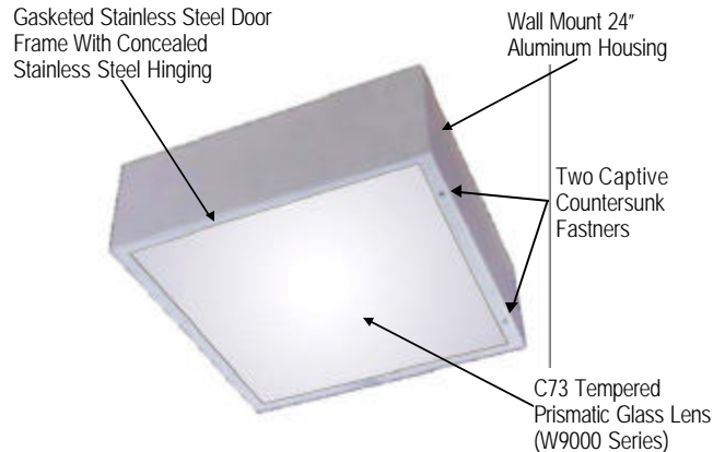
Wall Mount 24" Sq.
